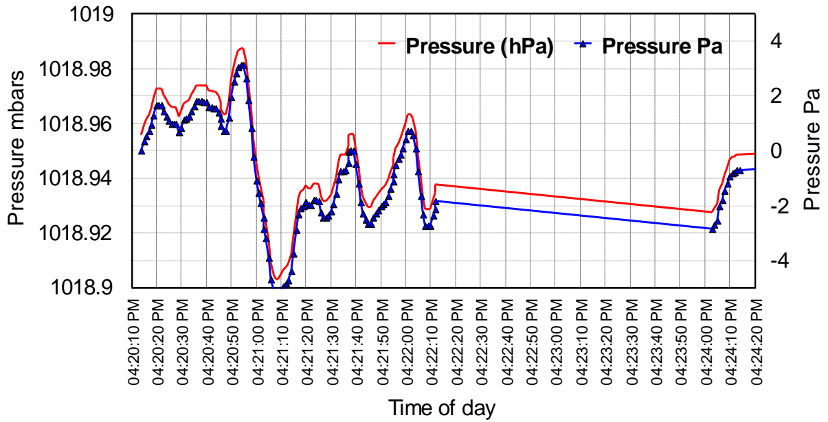
Illustrating normal variation of atmospheric pressure @ sea level (max around 1Pa/s)
