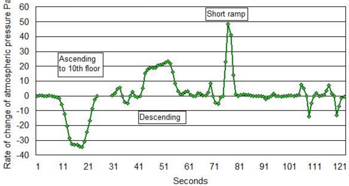
Riding elevator Change of Atmospheric pressure rate Pa/s
